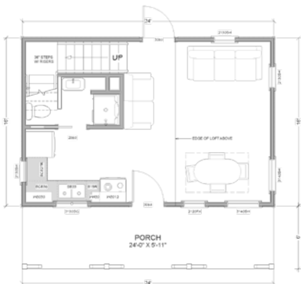
Main Floor
