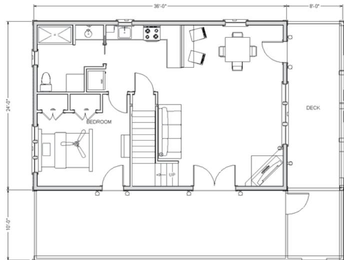
MAIN FLOOR
